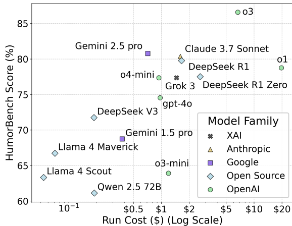
Figure 3: Benchmarking results on frontier models
